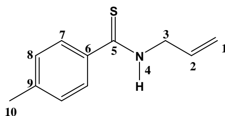
N-allyl-4-metilbenzotioamida (3d)
