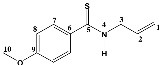
N-alil-4-metoxibenzotioamida (3c)
