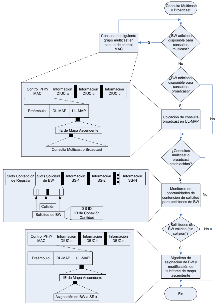
Figura 3.6. Consulta Multicast y Broadcast.
