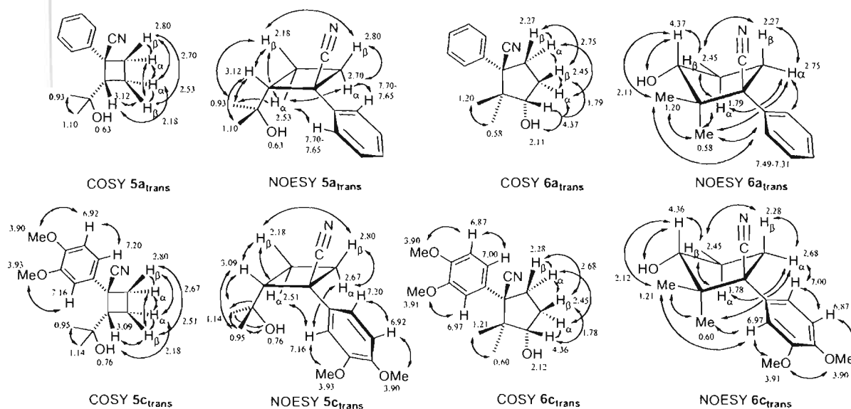
Scheme 4. COSY and NOESY correlations for compounds 5a trans , 6a trans , 5c trans , and 6c trans
