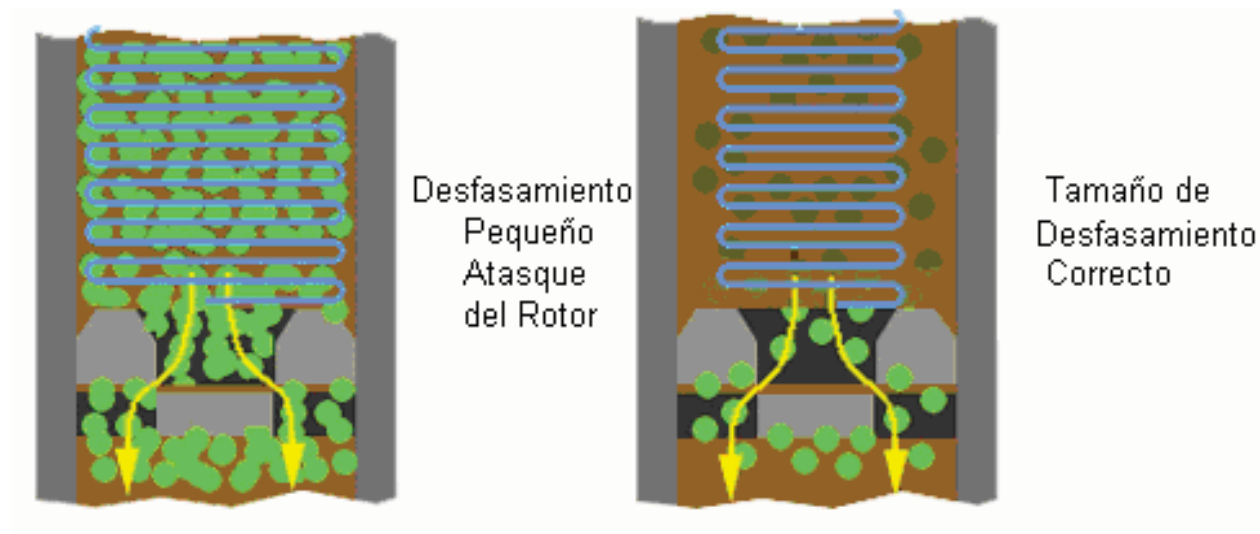
Figura III.16. Efectos de LCM. (Chagoya, 2007)
