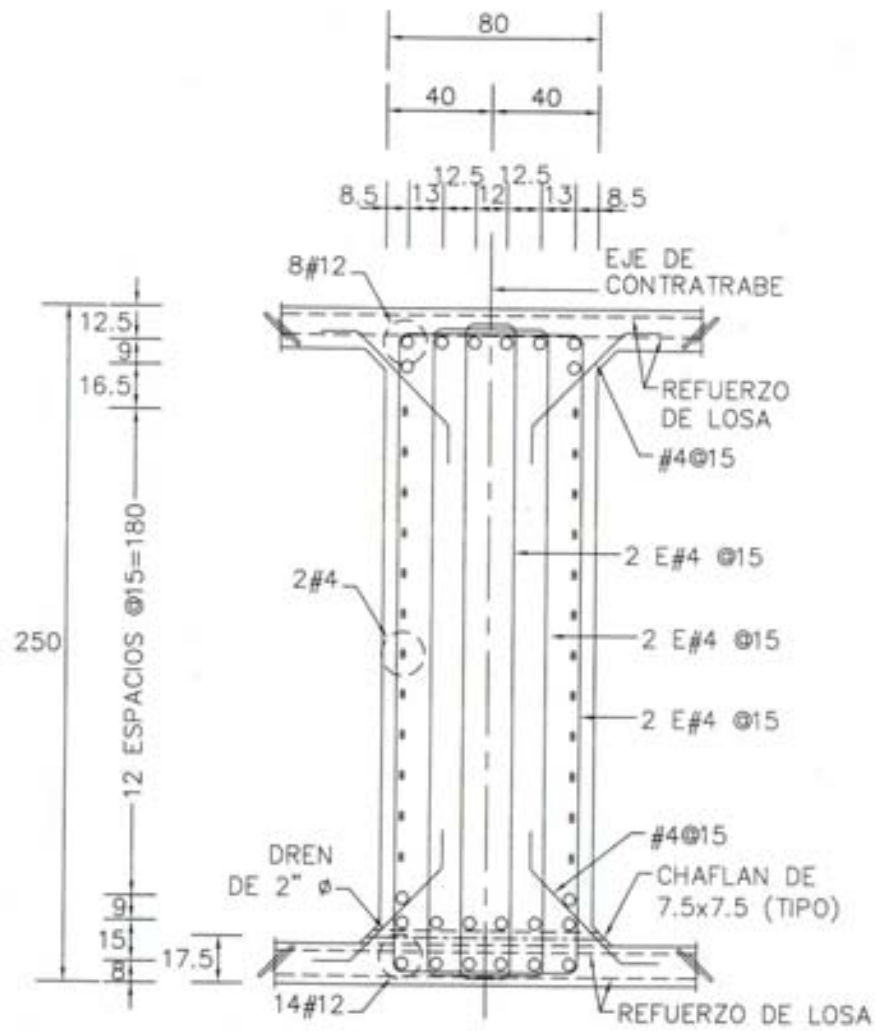
CT-5 CONTRABE
