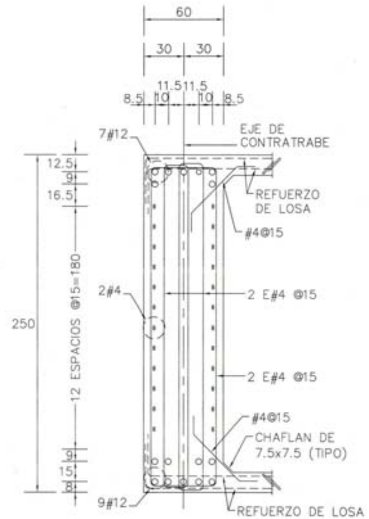
CT-4 CONTRATRABE
