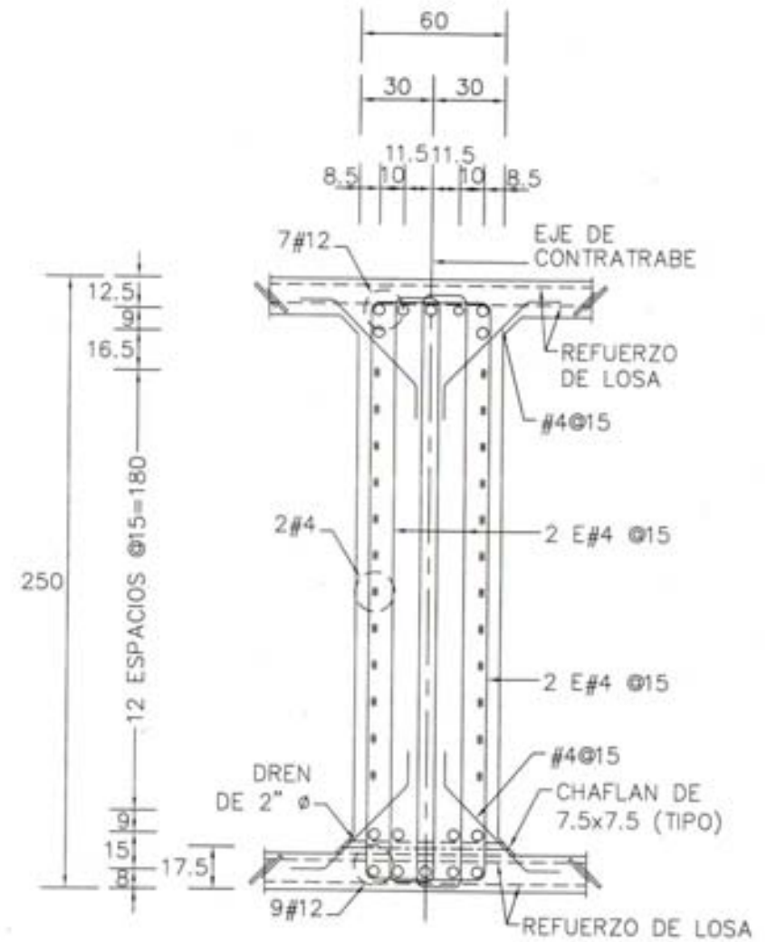
CT-6 CONTRABE
