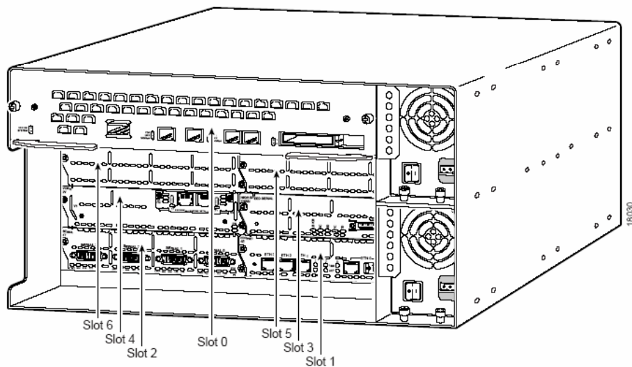
Figure 17-3: Cisco 3660 Router Rear View
