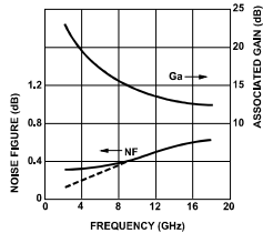
Figure 1. ATF-36077 Optimum Noise Figure and Associated Gain vs. Frequency for V_{GS} = 1.5 V, I_{DS} = 10 mA.
