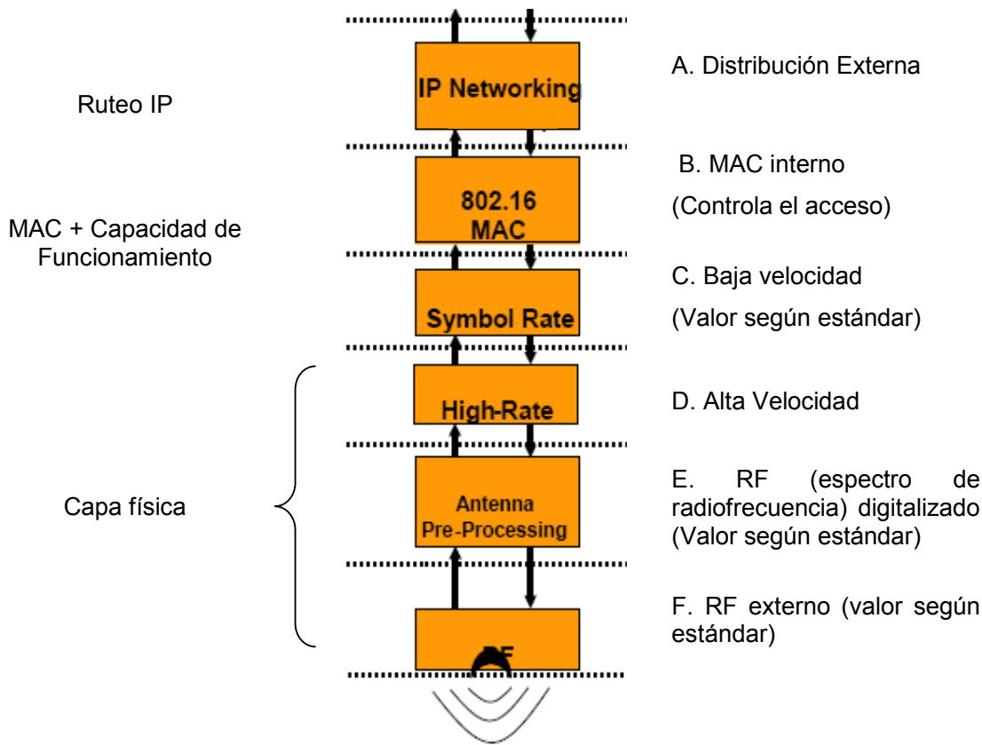
Figura 3-1 Modelo de Base Station BS.
