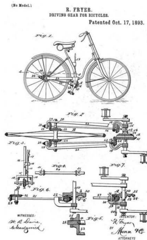
Fig. 3.3 Sistema de cardán (Shaft Drive).
