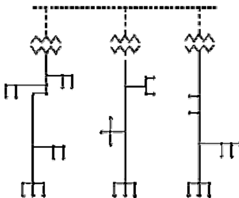
DIAGRAMA 3. RED RADIAL
