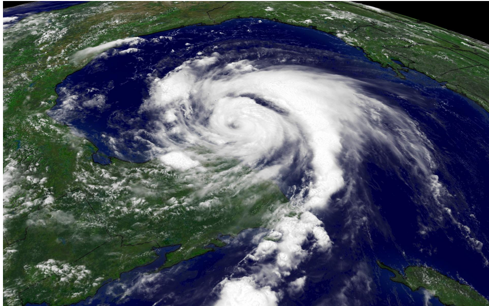
HURRICANE EMILY REGIONAL IMAGERY, 2005.07.18 AT 1815Z. CENTER POINT LATITUDE: 21:30:34N LONGITUDE: 89:48:38W.
