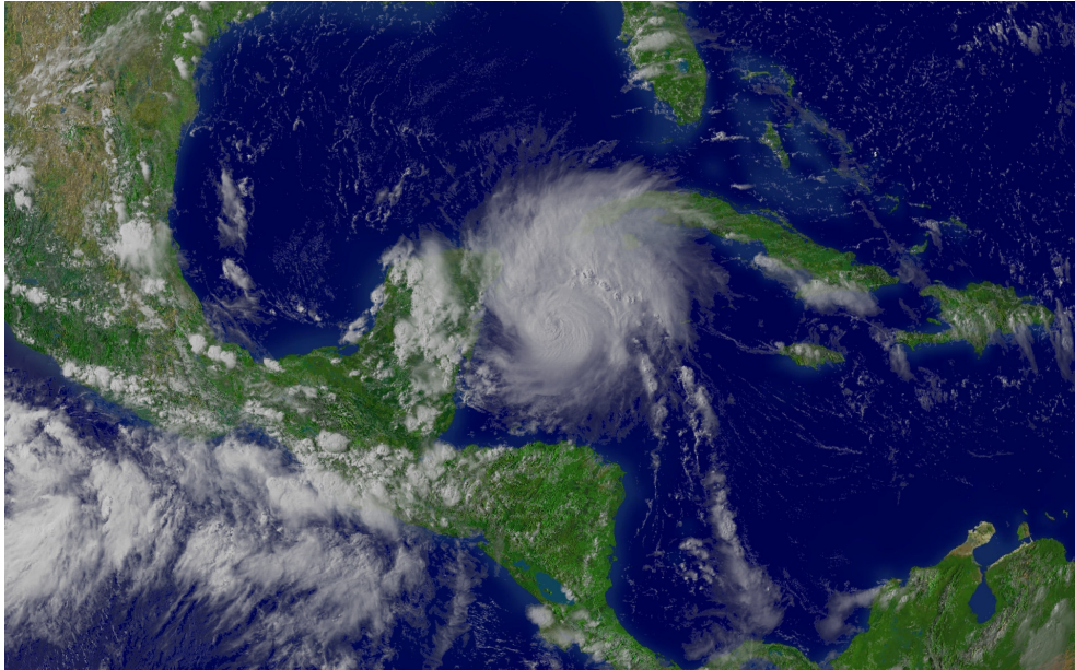
HURRICANE EMILY REGIONAL IMAGERY, 2005.07.17 AT 2115Z. CENTER POINT LATITUDE: 19:46:14N LONGITUDE: 85:17:55W.
