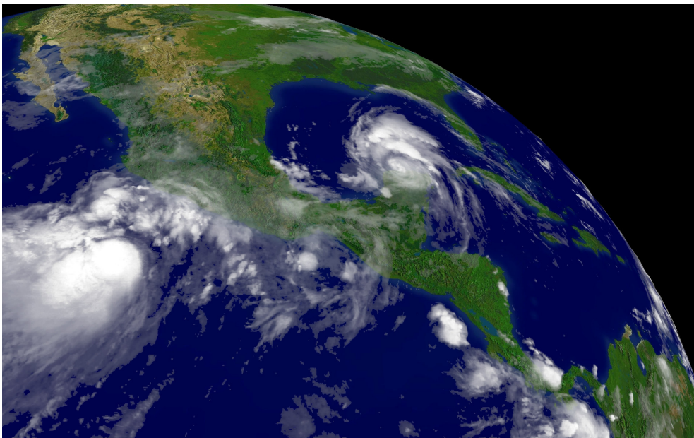
HURRICANE EMILY REGIONAL IMAGERY, 2005.07.18 AT 1245Z. CENTER POINT LATITUDE: 21:34:34N LONGITUDE: 88:56:36W.
