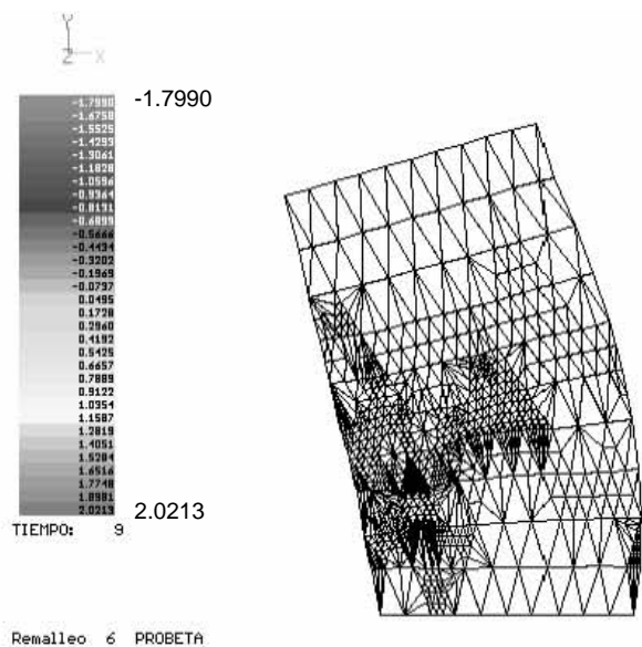
Figura A.14 Remalleo #6
