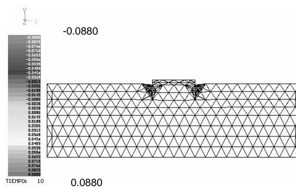
Figura A.40 Remalleo # 3
