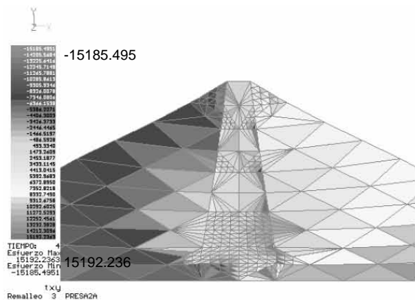
Figura A.59 Remalleo 3
