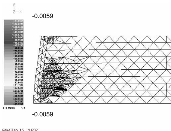
Figura A.76 Remalleo # 15
