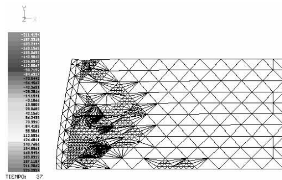
Figura A.78 Remalleo # 9
