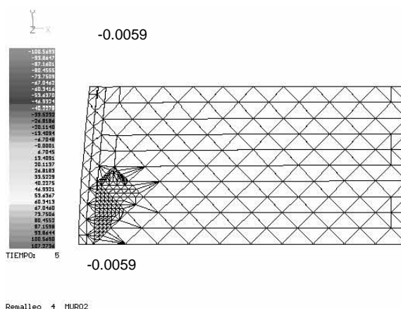
Figura A.74 Remalleo # 4
