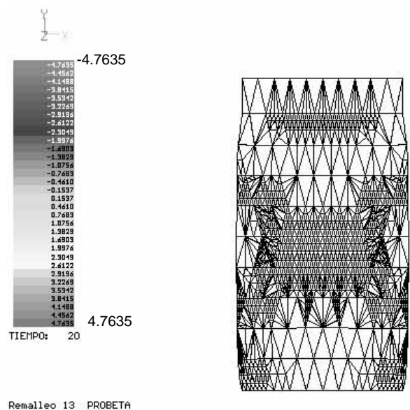
Figura A.23 Remalleo # 13
