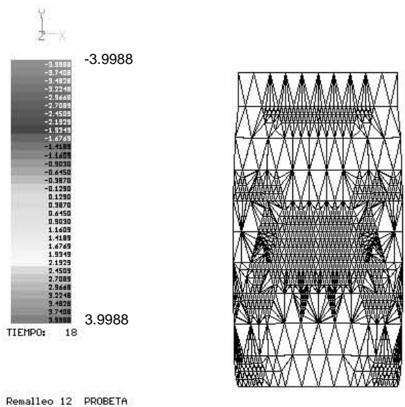
Figura A.22 Remalleo # 12
