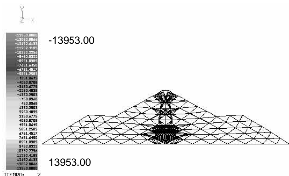
Figura A.50 Remallo # 2
