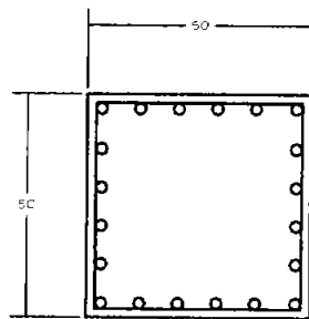
Columna C-1
