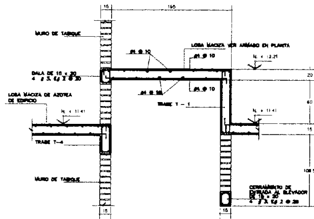
Corte 7-7'
