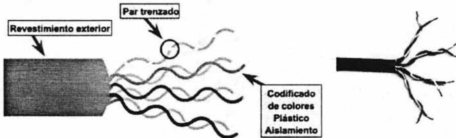
Figura II.12. Cable UTP
