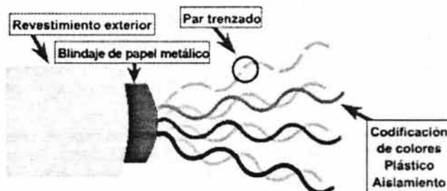
Figura II.15. Cable STP
