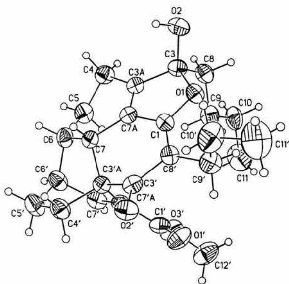
Figure 2. ORTEP-like view of compound 5.
