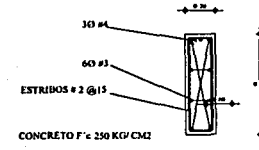
CONCRETO f_c = 250 \text{ KG/CM}^2 CONTRATRABE CT1 s/e
