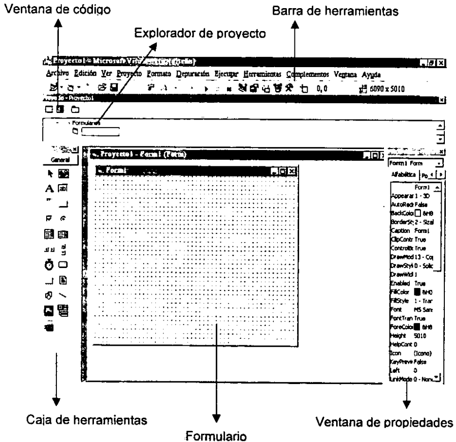
Figura 3.3.2. Visual Basic.
