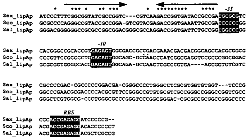
Fig. 5. Alignment of nucleotide sequences of the lipA promoter regions of S. exfoliatus M11 (Sex_lipAp), S. coelicolor A3(2) (Sco_lipAp) and S. albus G (Sal_lipAp). The conserved RBS and the -10 and -35 regions of the promoters are highlighted. Asterisks indicate bases that are conserved in all three species upstream of the -35 region. The position of the stem-loop structure in the S. exfoliatus M11 promoter region is indicated by arrows. Two small dots above the S. coelicolor sequence mark the transcriptional start point.
