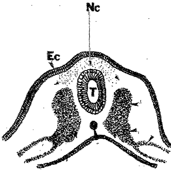
Fig. 2 Tubo Neural
