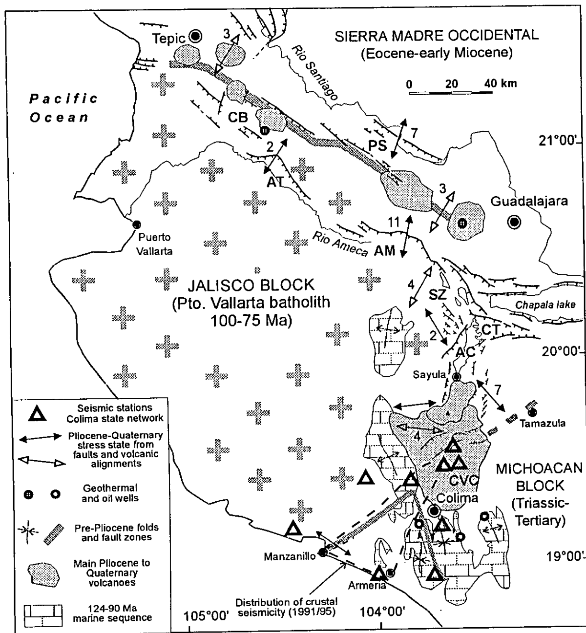
Figure 5.2.- Tectonic and stress map of Jalisco block and its boundaries. Latest Miocene to Quaternary faults in black. Double arrows are minimum horizontal stress orientations averaged for number of sites reported (after Rosas-Elguera, 1995). Main extensional structures mentioned in text: CB-Ceboruco, PS-Plan de Barrancas-Sata Rosa, AT-Amatan de Cañas, AM-Ameca, SZ-San Marcos-Zacoalco, AC-Amacueca, CT-Citala. CVC is Colima volcanic complex.
