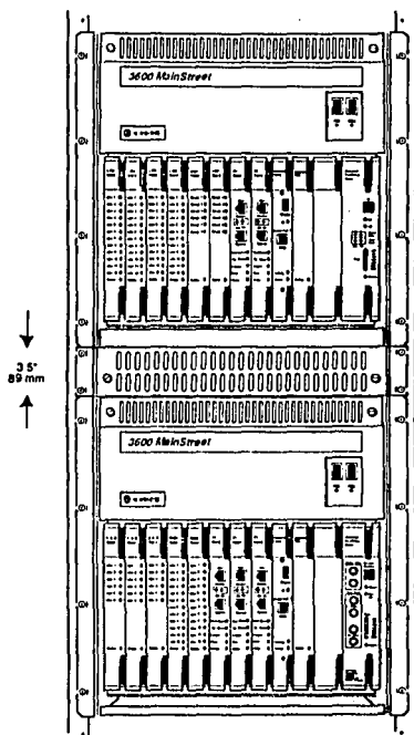
Figures 1-3: A Dual Shelf 3600 MainStreet with an Optional Heat Deflector
