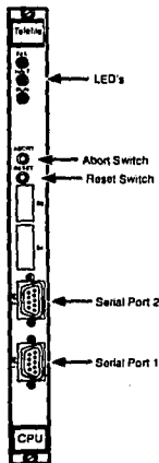
Figure 2-10. MVME-135 CPU module hardware components
