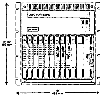
Figure 1-2: A Single Shelf 3600 MainStreet
