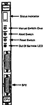
Figure 2-6. MVME-101 CPU module hardware components
