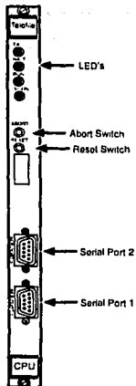
Figure 2-12. MVME-165 CPU module hardware components
