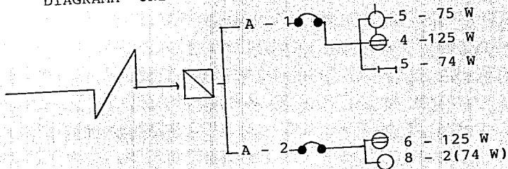
DIAGRAMA UNIFILAR
