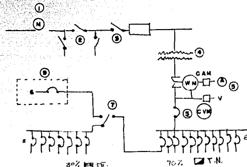
DIAGRAMA UNIFILAR
