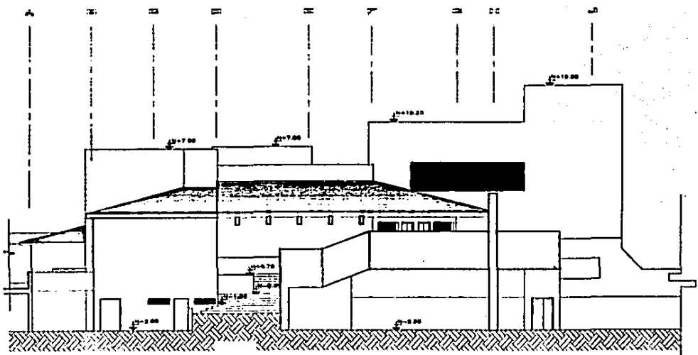
FACADENA D
