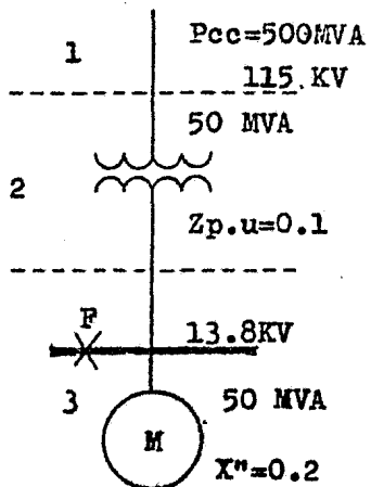
DIAGRAMA UNIFILAR
