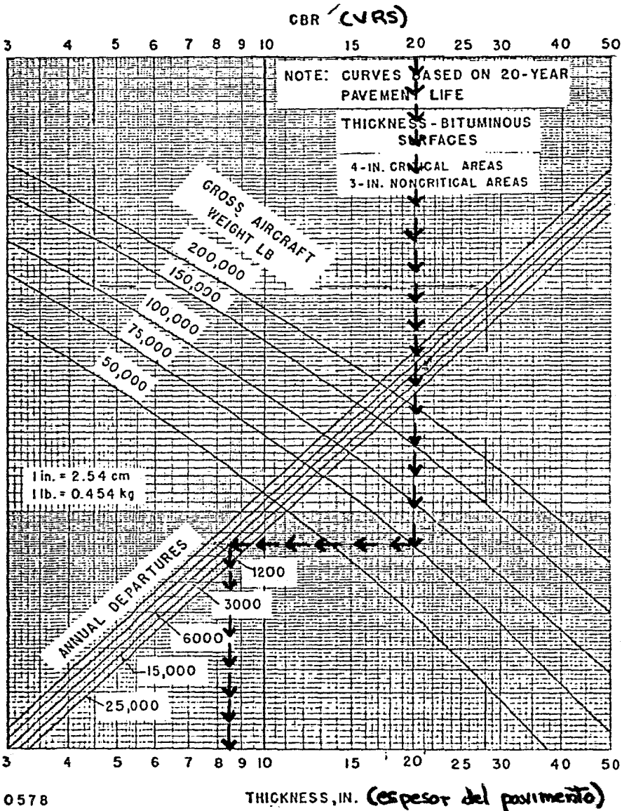
FIGURE 3-4. FLEXIBLE PAVEMENT DESIGN CURVES FOR CRITICAL AREAS, DUAL WHEEL GEAR (Rueda doble)
