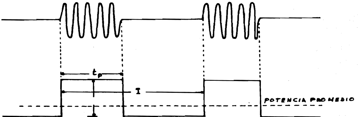
Fig. 2.14 Pulso simple.
